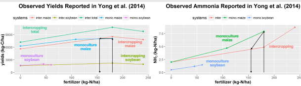
Fig.1 Field observations of a maize-soybean intercropping system in Sichuan, China (Yong et al., 2014). Intercropping allowed maize to yield the same as its monoculture counterpart using about 30 kg-N less fertilizer. Such reduction in fertilization eliminates the NH 3 emission by more than one-third of that from maize monoculture system.
