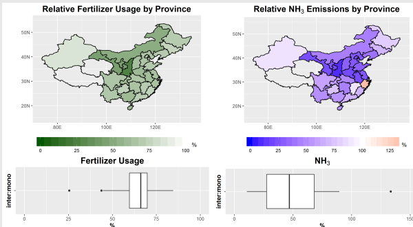
Fig.4 DNDC simulated nationwide adoption of maize-soybean intercropping in China. The maps show relative value of fertilizer required to achieve the same yield of maize under intercropping compared to fertilizer needed under monoculture (left) and their corresponding relative reduction in NH 3 emission (right). The boxplots summarize the provincial results. It is found that the mean fertilizer requirement is dropped to 64% of conventional usage and it correspondingly cuts 50% of NH 3 emission on average. Tibet and Xizang (blank regions on the maps), whose combined productions contribute to 0.01% of annual maize yields and 1% of soybean in China, are excluded from this study due to data insufficiency.
